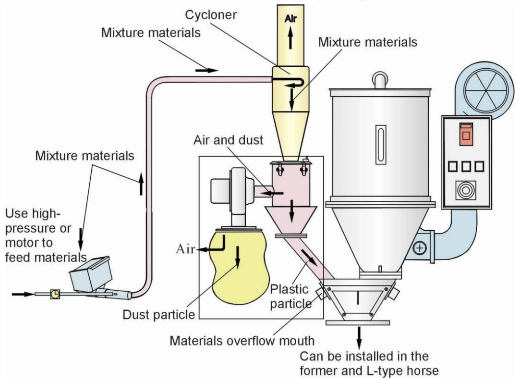
Picture 2-41: Dust separating System
